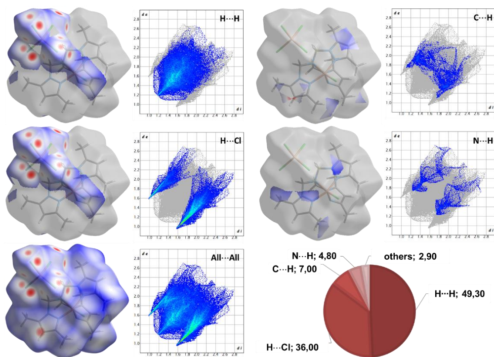
Fig. S1 3D Hirshfeld surfaces mapped with d_{\text{norm}} with corresponding 2D fingerprint plots and the percentage of non-covalent interactions in complex 1.
