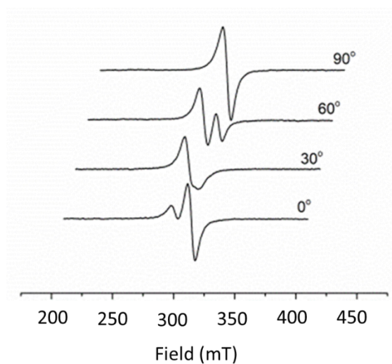
Fig. S6 The experimental EPR spectra of single crystal of complex 1 recorded at T = 5\text{K} at different angles of the external magnetic field with respect to the crystal.
