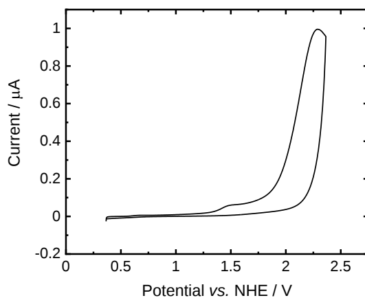
Fig. S8 Cyclic voltammogram of the scorpionate ligand recorded under ambient air atmosphere in acetonitrile solution containing 0.1 M NBu 4 PF 6 with the scan rate 1 V/s.
