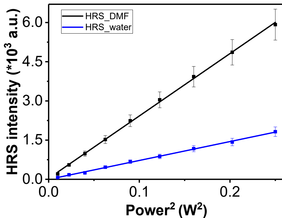
Figure S11: Plot of the HRS intensity for DMF and water as a function of (laser power) 2 (at 800 nm laser excitation).
