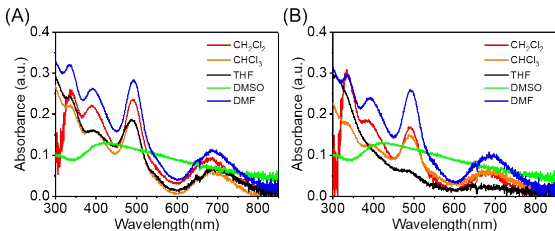
Figure S1. Absorption spectra of \text{Ag}_{25}(\text{SR})_{18} in \text{CH}_2\text{Cl}_2 , \text{CHCl}_3 , THF, DMSO, DMF after fresh preparation (A) and after 1 day (B). \text{Ag}_{25}(\text{SR})_{18} concentration: 2.74\mu\text{M} . \text{Ag}_{25}(\text{SR})_{18} in DMSO degraded within 10 mins; \text{Ag}_{25}(\text{SR})_{18} in THF degraded after 1 day; \text{Ag}_{25}(\text{SR})_{18} in \text{CH}_2\text{Cl}_2 , \text{CHCl}_3 , DMF can retain absorption feature after 1 day. (with SR=DMBT).
