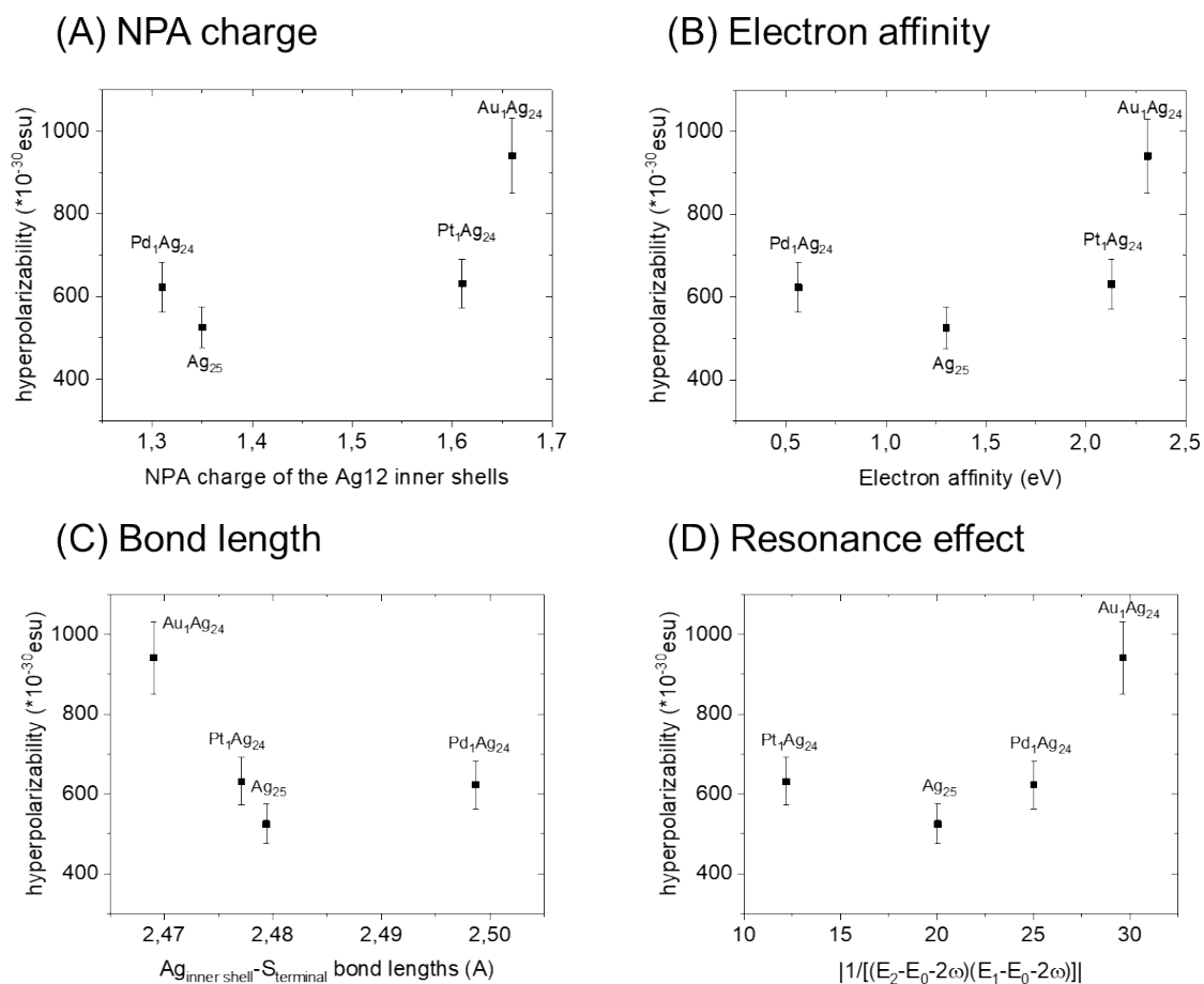
Figure S6. Plots of hyperpolarizability ( \beta(2\omega) ) values and some relevant properties of \text{M}_1\text{Ag}_{24}(\text{SR})_{18} nanoclusters, leading to charge transfer and resonance effects. Relevant properties: (A) NPA charge of the Ag12 inner shells; (B) Electron affinity of Pd/Ag/Pt/Au; (C) \text{Ag}_{\text{inner shell}}-\text{S}_{\text{terminal}} bond lengths average; (D) Resonance factor |1/[(E_2-E_0-2\omega)(E_1-E_0-2\omega)]| . E_1 , E_2 represent the energy of 2 absorption bands of \text{M}_1\text{Ag}_{24}(\text{SR})_{18} nanoclusters, and E_0 represents the energy of excitation light. Charge factors are obtained from previous report. 3
